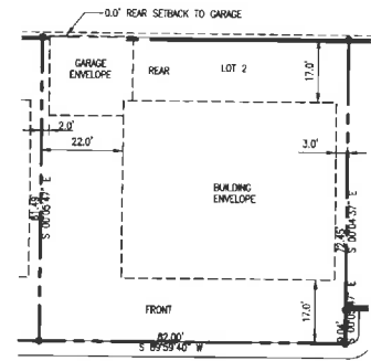
TYPICAL LOT PLAN: SCALE: 1"=20'
